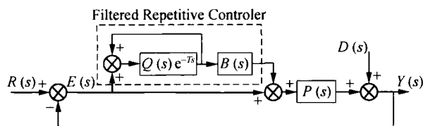
Fig. 3 Plug-in RC system diagram
